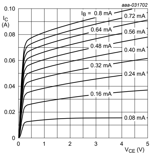
Fig. 11. NHDTC124ET-Q: Collector current as a function of collector-emitter voltage; typical values
