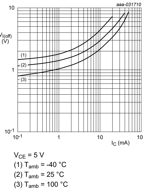
Fig. 19. NHDTC144ET-Q: Off-state input voltage as a function of collector current; typical values
